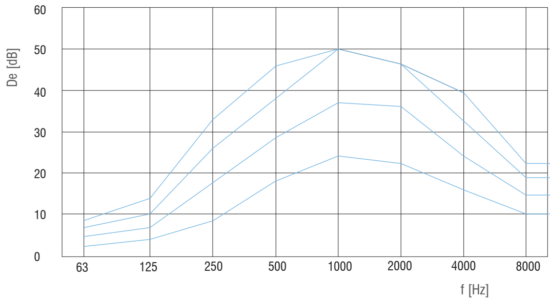
Attenuation diagram, type PZ 200/100
