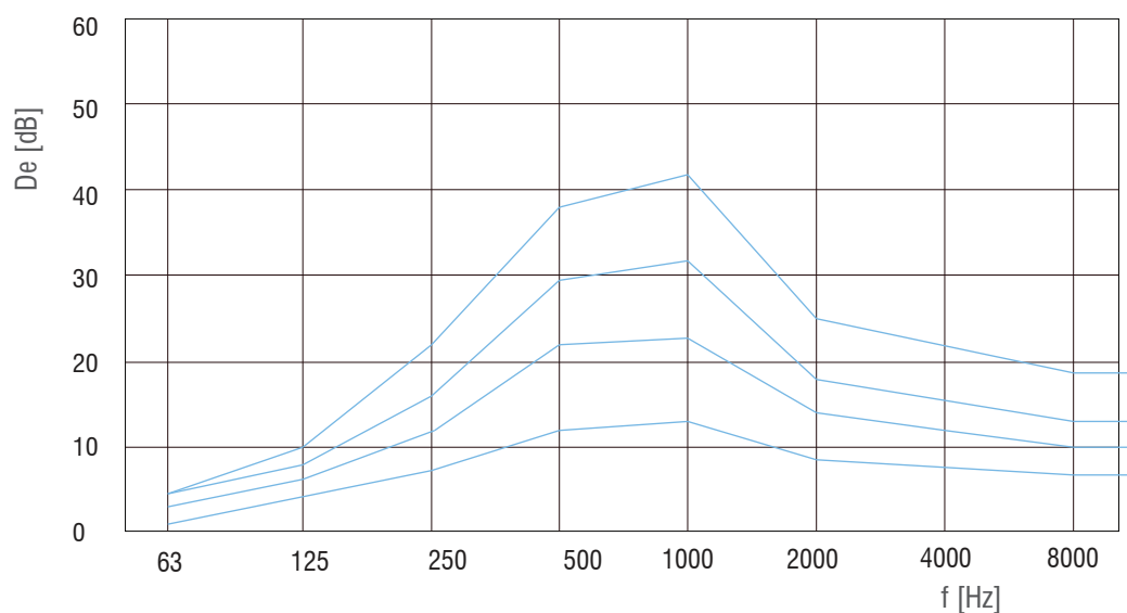
Attenuation diagram, type PZ-R 100/100
