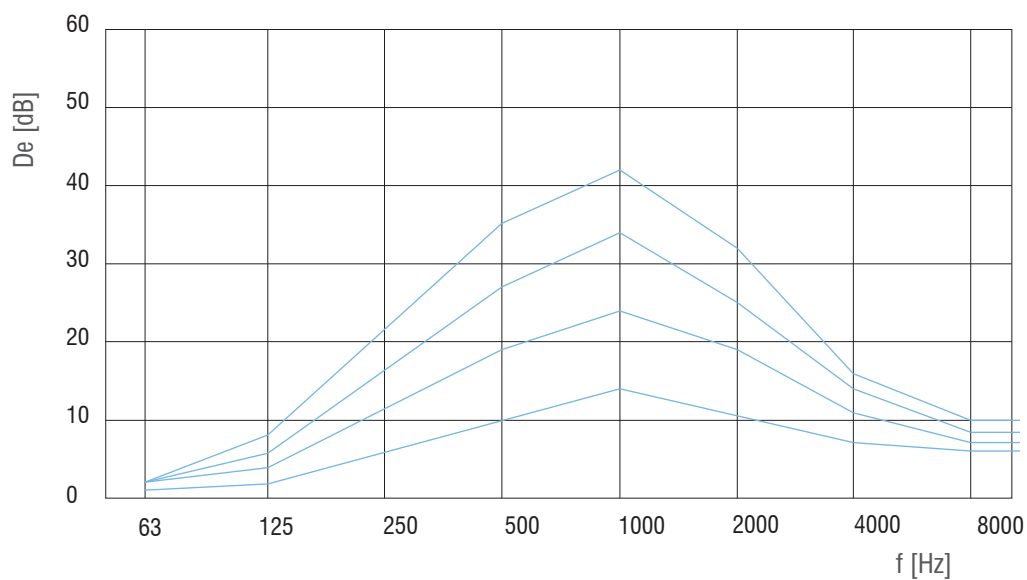
Attenuation diagram, type PZ 200/200
