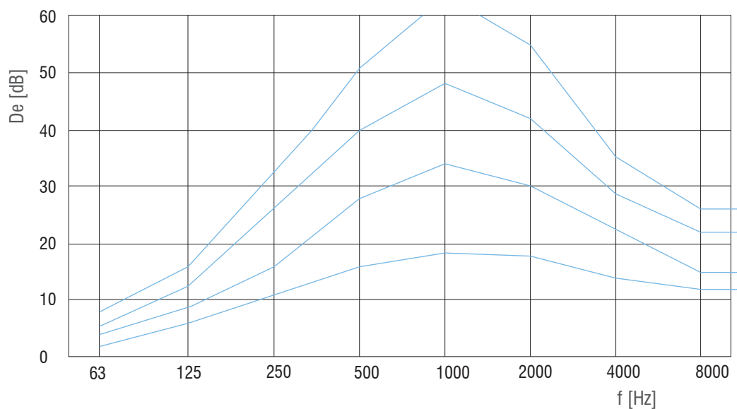
Attenuation diagram, type PZ-R 100/50
