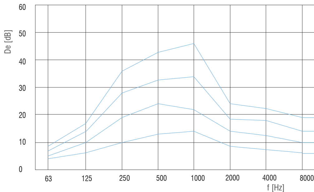
Attenuation diagram, type PZ-R 200/100
